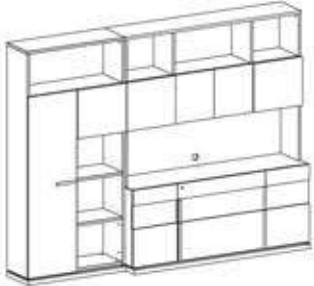
LIBRARY COMPOSITION 5 PJMN0804 inch W 110" D 21" H 84" cm L 279,6 P 52,7 H 213,4 Crts 8 kg 314 m 3 1,655
