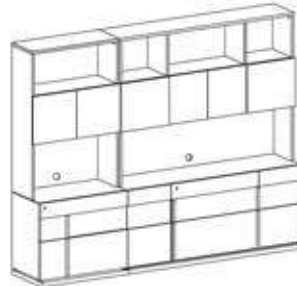
LIBRARY COMPOSITION 7 PJMN0806 inch W 106" D 21" H 84" cm L 269,6 P 52,7 H 213,4 Crts 8 kg 330 m 3 1,872
