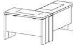
DESK COMPOSITION 3 PJMN0818 Desk + Return desk inch W 47" D 71" H 30" cm L 120 P 175 H 76 Crts 2 kg 90 m 3 0,286
