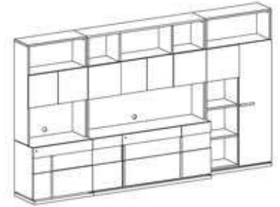
LIBRARY COMPOSITION 4 PJMN0803 inch W 146" D 21" H 84" cm L 369,6 P 52,7 H 213,4 Crts 11 kg 430 m 3 2,265
